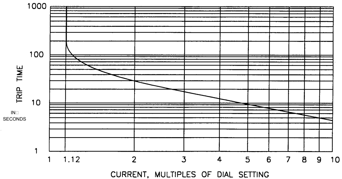
OVERLOAD TRIP TIME VS CURRENT CURVE TRIP CLASS 10
